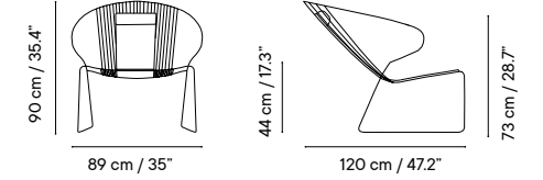
iSi 9143 Lounge cushion Icons: chair, outdoor, indoor
